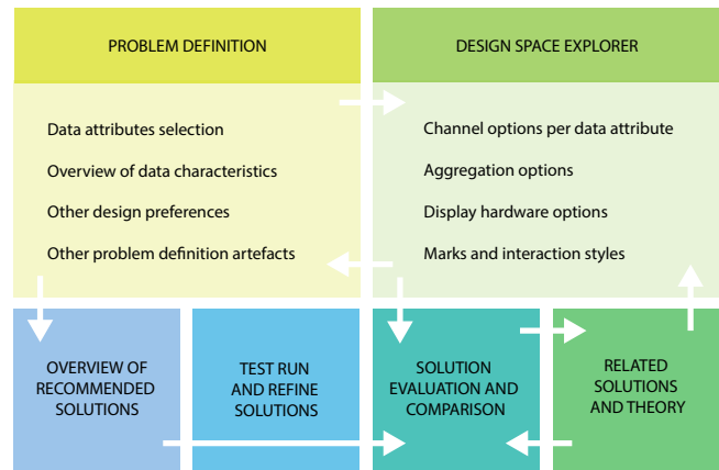
Figure 2: Components of a visionary system for designers that integrates recommendation algorithms into a more holistic workspace, allowing for iterative development of designs.
